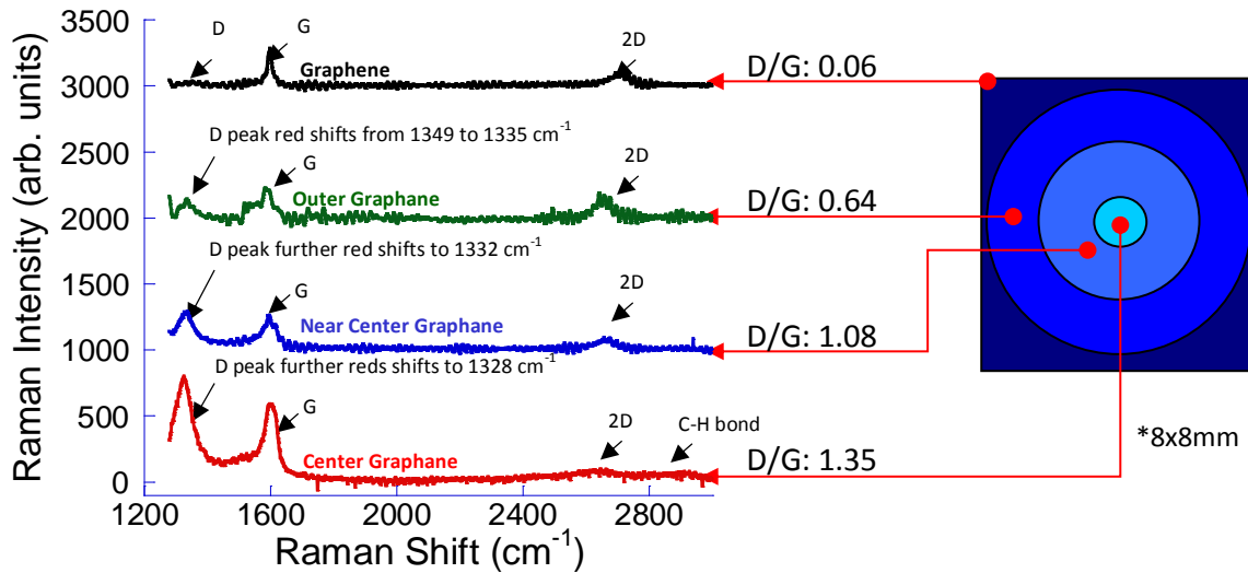
Figure 3.9 Hydrogenation gradient observed with electrochemical hydrogenation of epitaxial graphene
