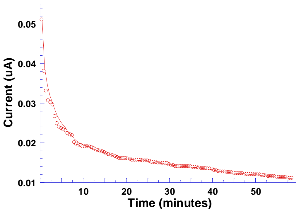
Figure 3.6 I vs. t curve for electrochemical hydrogenation of graphane. About 1 monolayer of hydrogen was calculated from the total integrated charge for 2 monolayers of graphane
